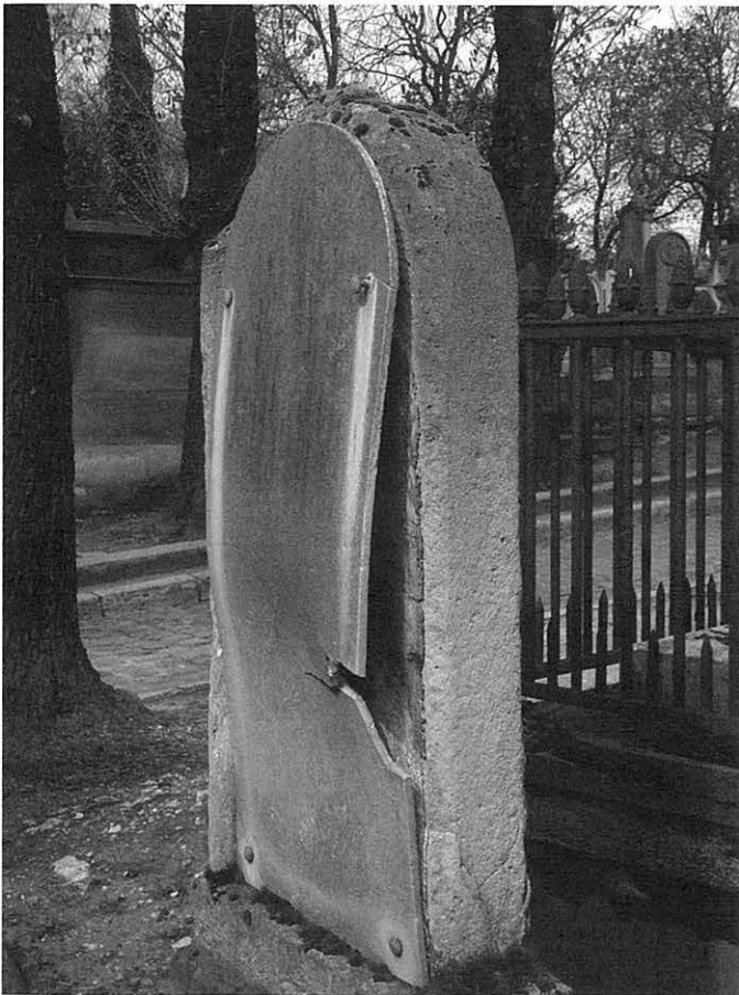
Marble deterioration on a monument in Montmartre cemetery, Paris. (Photo: Brent Gelk)
