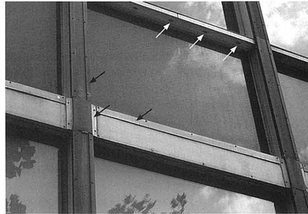
Remedial aluminum covers and weep hole plugs, c. 1952
