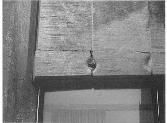
The thin stone panels on the Laird Bell Law Quadrangle are deteriorated due to corrosion of the steel anchors.
