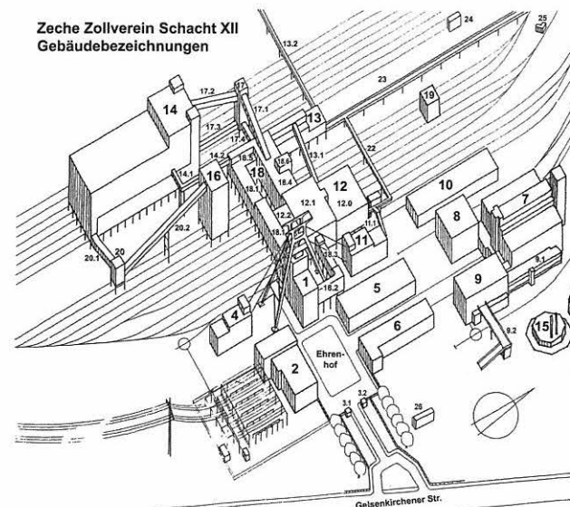
Axonometric drawing of the Shaft XII site.
